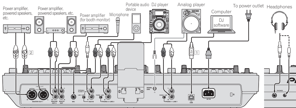
Rear panel
