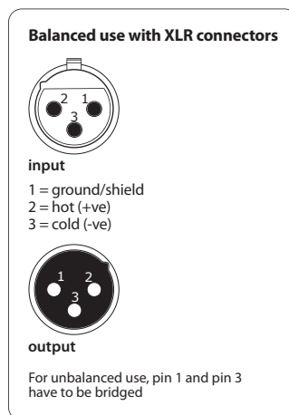
Fig. 8.1: XLR connector
