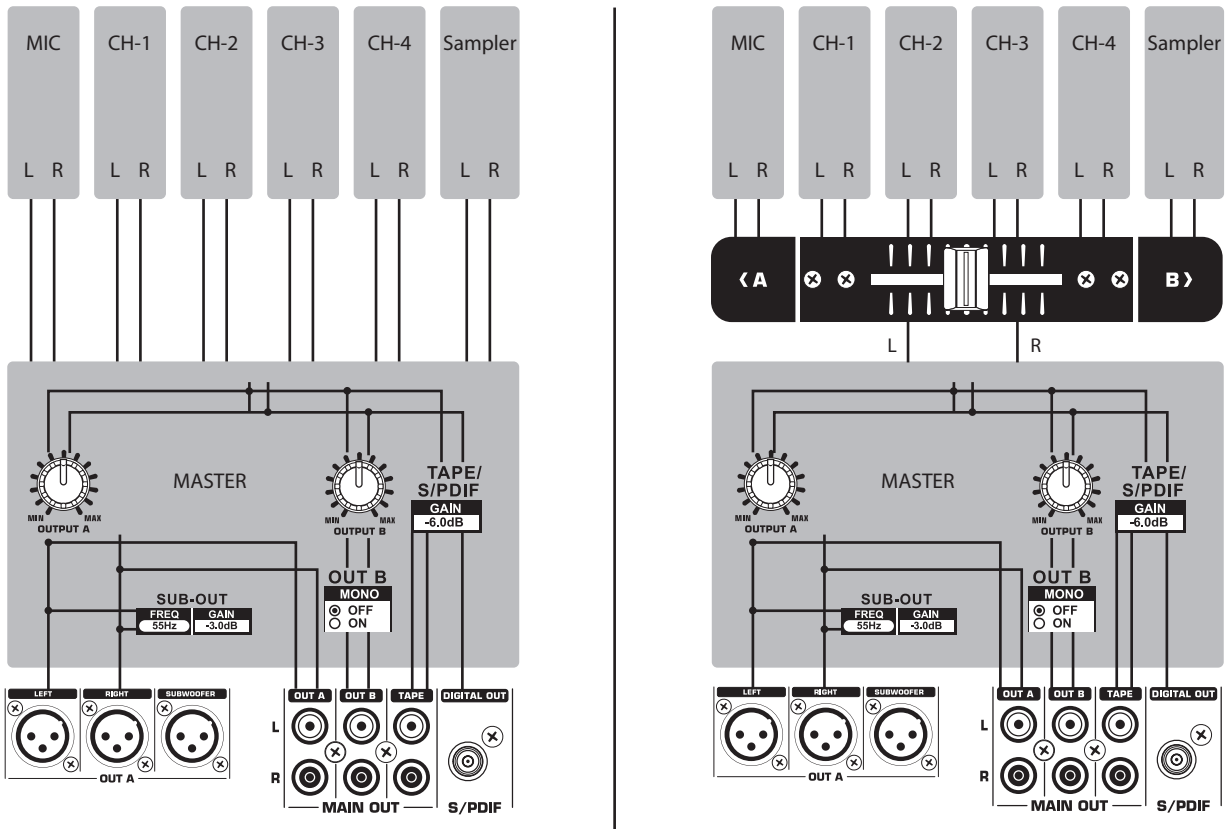
Fig. 10.2: Mixer routings
