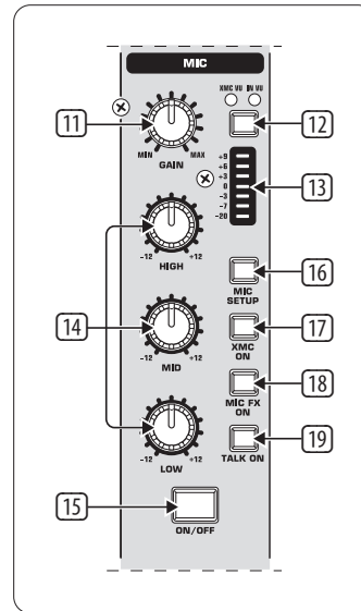
Fig. 2.2: Microphone channel
